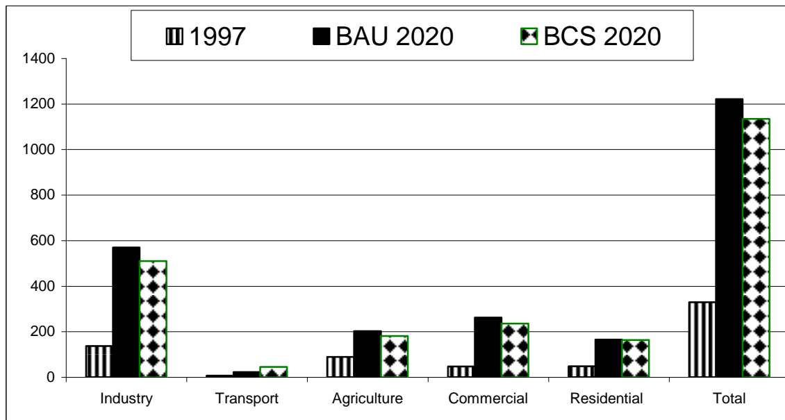
Figure 3: Project Power Demand in India by 2020 (in TWh)
